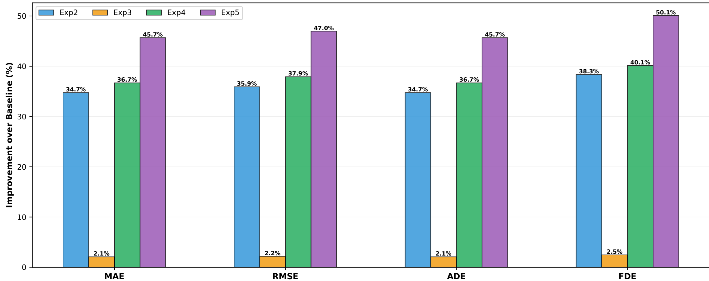
Performance Improvement Relative to Exp1 (Baseline GRU)
